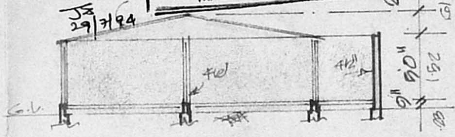
SECTION-CD
