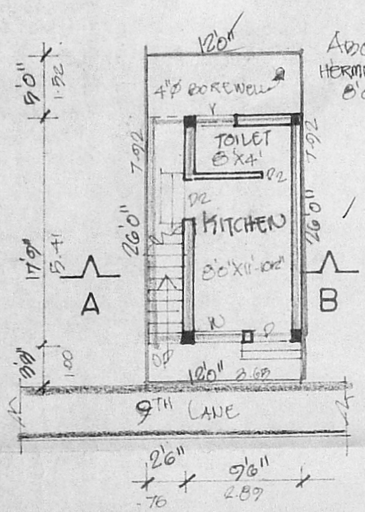
SITE PLAN / G.F. PLAN
