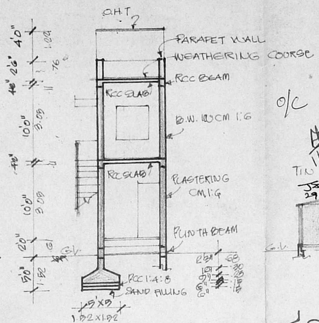
SECTION-AB
